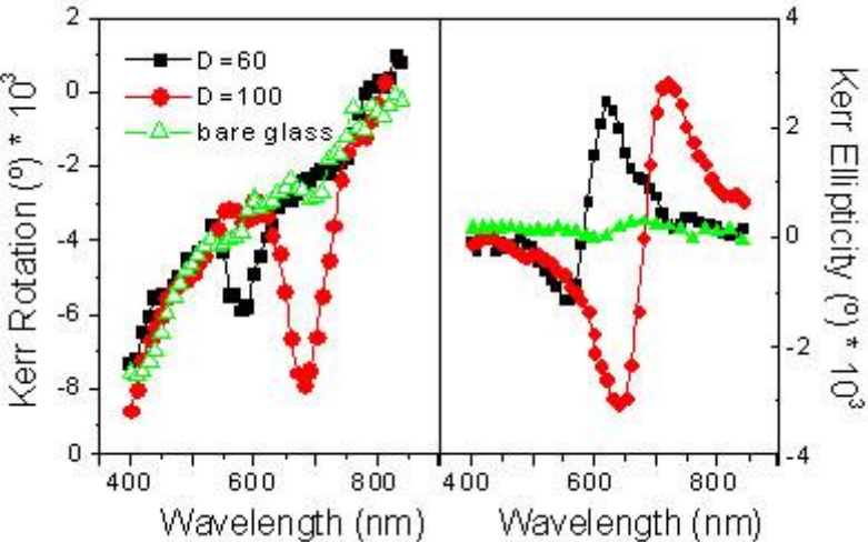
Fig. 1: MO Kerr rotation and ellipticity of gold nanodiscs
