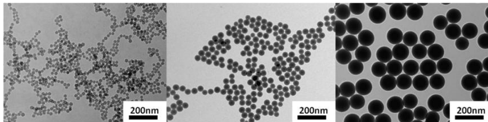
Fig.1 Representative TEM images of three sizes of SiO 2 NPs: 25, 60 and 115 nm.
