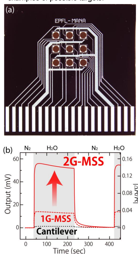
Fig. 2: (a) Photograph of the fabricated 2G-MSS chip with a 2D array. (b) Obtained output signals from each sensor.
